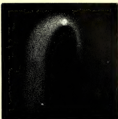
June 28.
